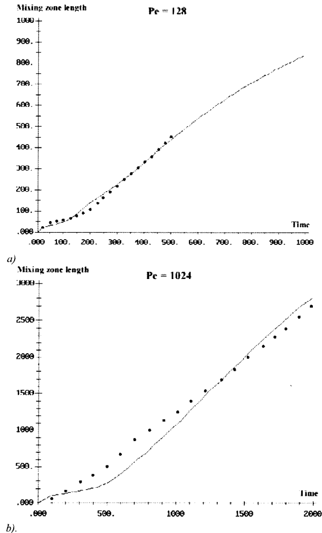
Fig. 9 a. Mixing length vs. time for Pe=128 . The dotted line is simulation published in (De Wit & Homsy, 1997). The solid line relates to our simulations Fig. 9 b. Mixing length vs. time for Pe=1024 . The dotted line is simulation published in (De Wit & Homsy, 1997). The solid line relates to our simulations.
