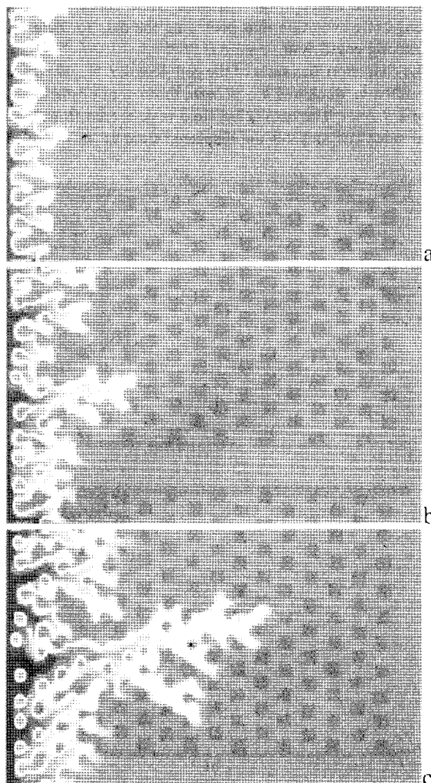
Fig. 17. Saturation maps for viscous fluids displacement: viscosity ratio M=84 , random obstacles, dimensionless time \tau = t - U / L : a- 0.053; b- 0.089; c- 0.166.
