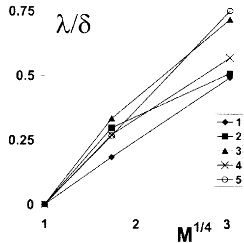
Fig. 4. The mean dimensionless thickness of fingers as a function of viscosity ratio in the power 1/4 for different experiments: Curve 1 - U=1 cm/s, \delta=1.2 mm; Curve 2 - U=1 cm/s, \delta=3.7 mm; Curve 3 - U=2.75 cm/s, \delta=1.2 mm; Curve 4 - U=2.75 cm/s, \delta=3.7 mm; Curve 5 - U=5 cm/s, \delta=1.2 mm.
