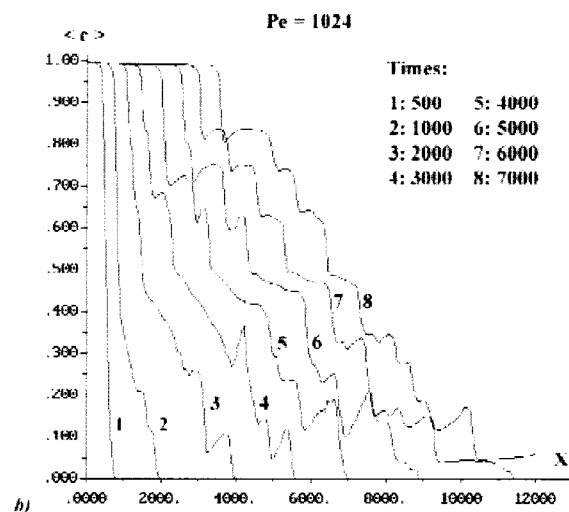
Fig. 11. Averaged by width concentration profiles for successive times: a - Pe=128 , M=3 ; b - Pe=1024 , R=3 .
