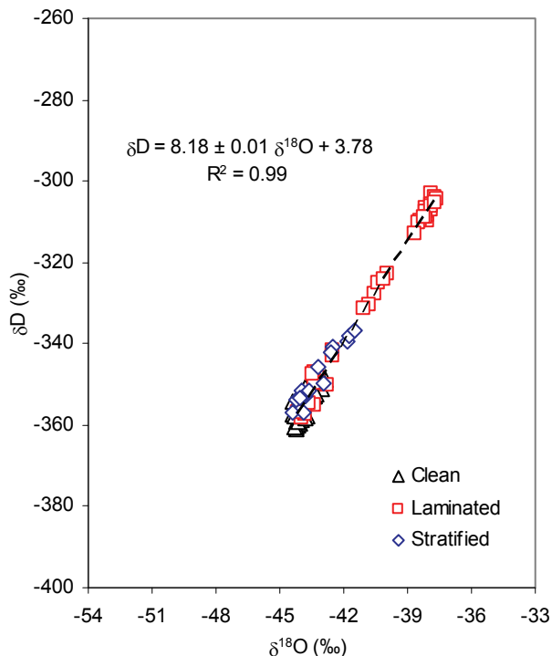
Figure 1. Co-isotopic plot of basal ice samples from Taylor Glacier. Samples plot on a slope of 8.18.
