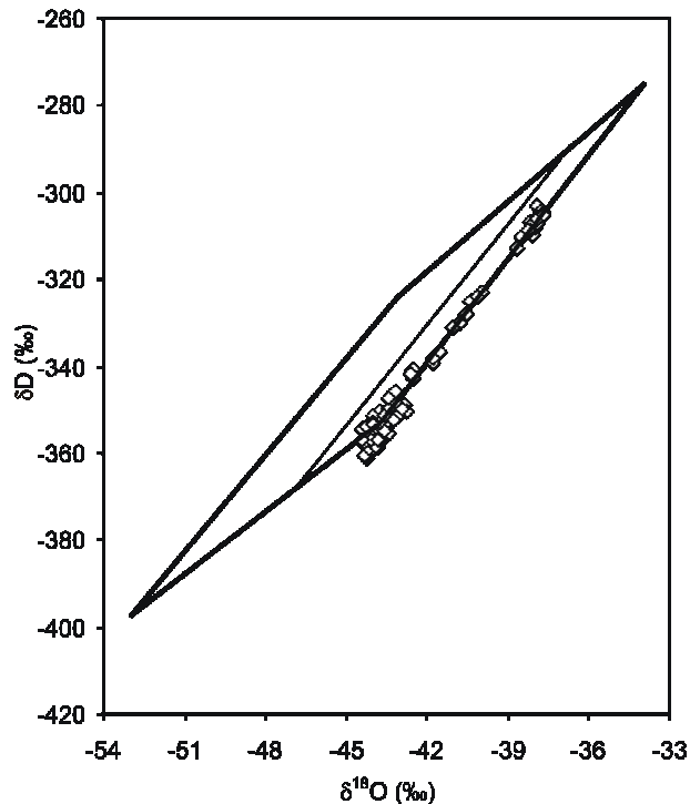
Figure 2. Theoretical freezing envelope for Taylor Glacier based on highest and lowest isotopic pairs from Taylor Dome meteoric samples. Basal ice samples (diamonds) plot on the extreme right of the envelope, whereas meteoric water line (light line) is offset by 3‰.
