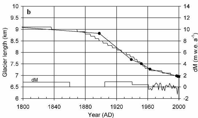
Fig. 5. Result of the dynamic calibration for SOF (a) and MAK (b) profiles. The observed glacier stands are marked by black dots. The lower solid line is the reconstructed mass-balance history.
