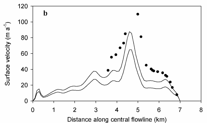
Fig. 6. Comparison between observed (dashed line/black dots) and modelled (solid lines) glacier elevation (a) and surface velocities (b) for AD 2000. The upper (lower) solid line corresponds to SOF (MAK) results.
