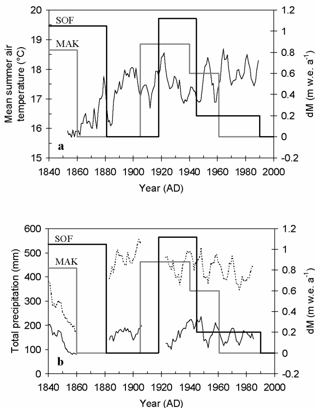
Fig. 9. Comparison between the 5 year running means of the Barnaul summer air-temperature (a) and precipitation (b) record and the reconstructed SOF (thick black line) and MAK (thick grey line) mass-balance histories. For the latter, annual mass-balance variations between 1962 and 1999 are not shown and are replaced by their mean value of 0 \text{ m w.e.a}^{-1} . The dashed line represents annual precipitation.
