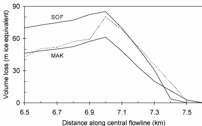
Fig. 7. Comparison between observed (dashed line) and modelled (solid lines) volume loss in the glacier front zone, 1952–2000. Results are shown for forcings with the SOF and MAK profiles.
