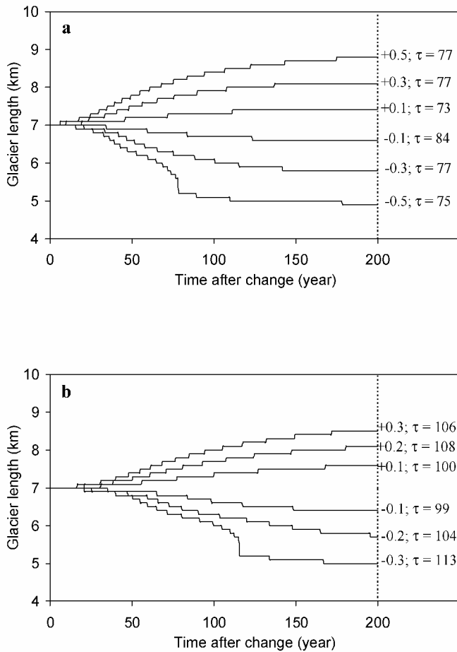
Fig. 4. Reaction of the glacier front position to a stepwise change in surface mass balance of given magnitude (in m w.e. a -1 ) for SOF (a) and MAK (b) profile. The corresponding response time \tau is given in years.
