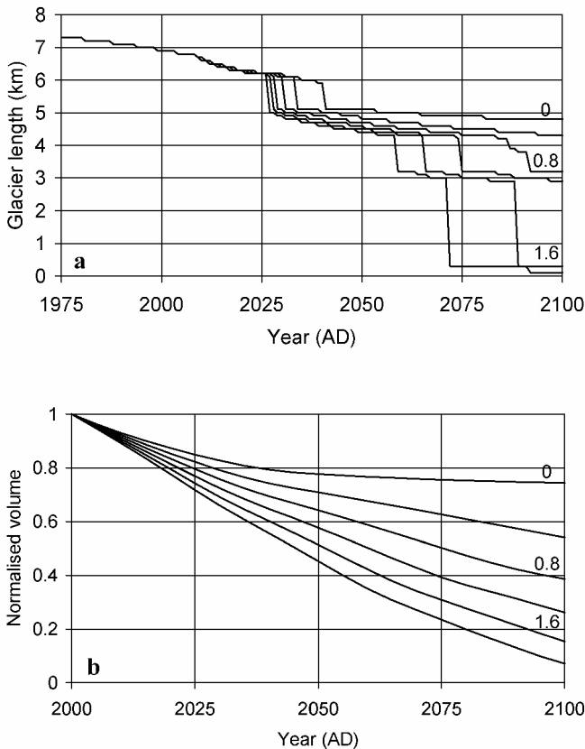
Fig. 10. Projected retreat (a) and volume loss (b) of Sofiyskiy glacier under six future climate scenarios (see text) for SOF. Labels indicate the magnitude of the corresponding total mass-balance drop. Volume is normalized with the 2000 volume. With MAK forcing, retreat and volume loss are slightly larger.
