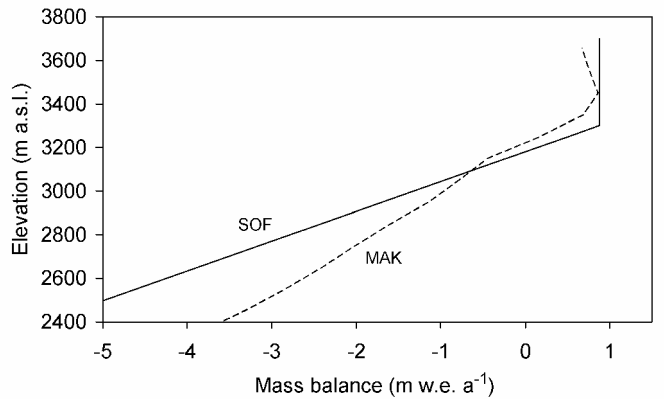
Fig. 3. Mass-balance reference profiles of Sofiyskiy glacier (solid line, SOF) and Maliy Aktru glacier (dashed line, MAK) (Pattyn and others, 2003).
