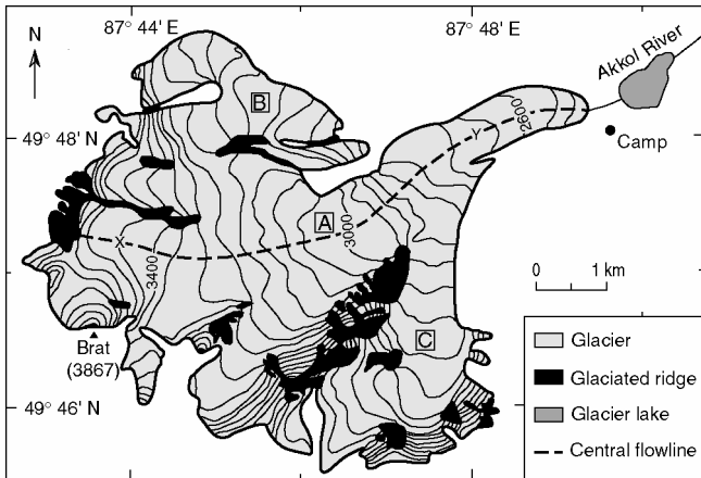
Fig. 2. Contour map of Sofiyskiy glacier based on a 1952 topographic map. At present, basins B and C are no longer connected with the main ice flow. “Camp” indicates the position of the glacier camp.
