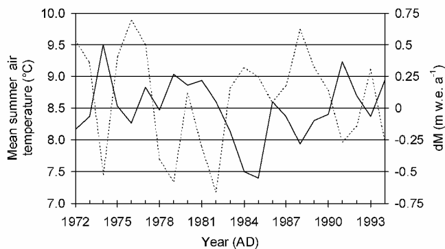
Fig. 8. Mean summer air temperature at Aktru station (solid line) and average annual mass-balance variation relative to the reference profile for Maliy Aktru glacier (dashed line) for the 1972–94 period.
