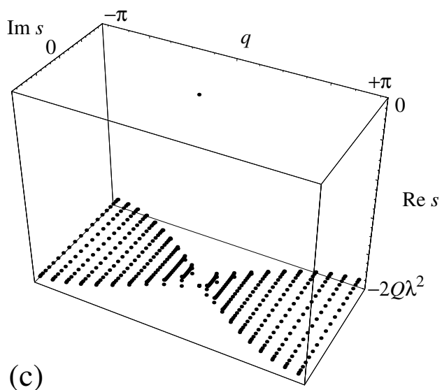
FIG. 4: Complete spectrum of the eigenvalues s_{q\theta} versus the wavenumber q for the Redfield superoperator (16)-(17). The eigenvalues are given by Eq. (108) in terms of the eigenvalues \mu_{q\theta} depicted in Figs. 1-3 at given values of the wavenumber. The size of the chain is here N = 21 . The parameter values are: (a) \frac{A}{Q\lambda^2} = 0.4 ; (b) \frac{A}{Q\lambda^2} = 0.7 ; (c) \frac{A}{Q\lambda^2} = 10 .
