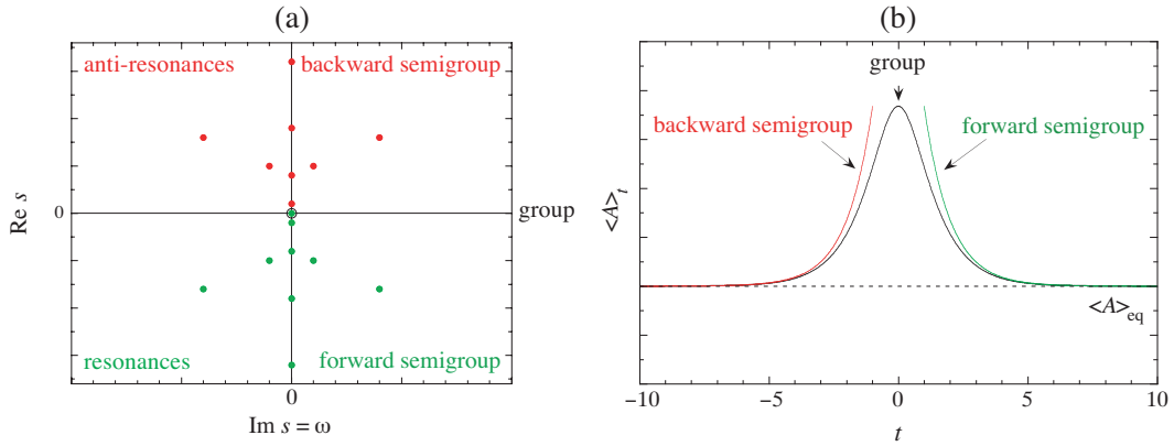
FIG. 7: (a) Pollicott-Ruelle resonances and anti-resonances in the complex plane of the rate s = -\gamma + i\omega . (b) Time decay of the mean value of an observable A toward its equilibrium value according to the group of time evolution and asymptotic expansions of the forward and backward semigroups valid for either positive or negative times.
