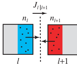
FIG. 8: Schematic representation of the mechanism generating the current (32) in the multibaker map.
