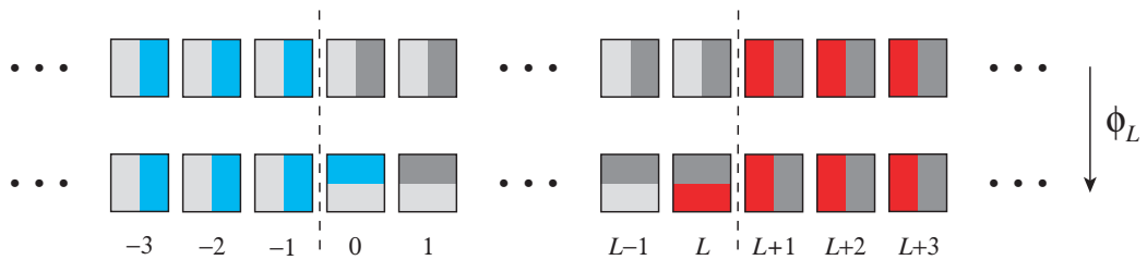
FIG. 4: Finite chain of the multibaker map connected to two particle reservoirs at l < 0 and L < l .
