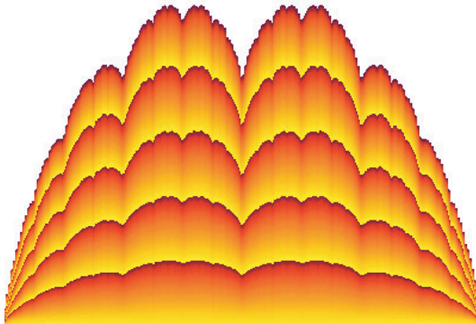
FIG. 5: Multiples xT(y) of the Takagi function versus the variable y , representing the singular part of the cumulative function of the nonequilibrium steady state of the dyadic multibaker map. The color changes for different values of the variable x .
