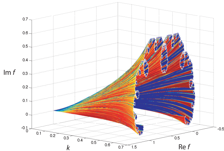
FIG. 6: The diffusive modes of the multibaker map represented by their cumulative function depicted in the complex plane ( \text{Re } f_k, \text{Im } f_k ) versus the wavenumber k .
