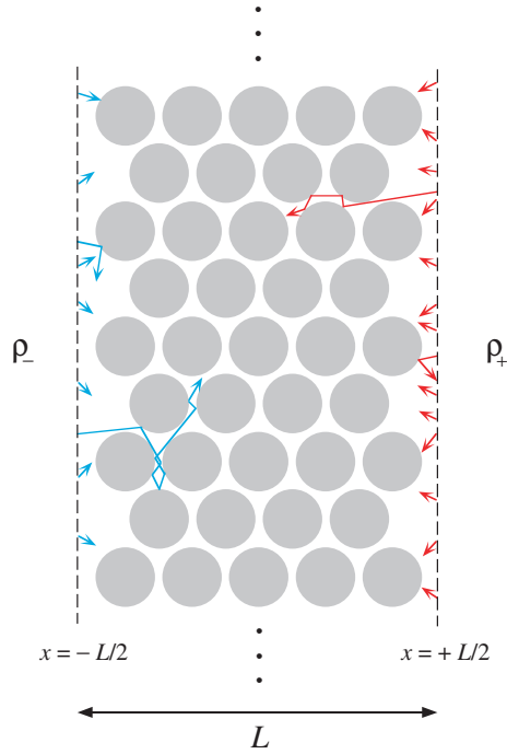
FIG. 3: Slab of the hard-disk Lorentz gas in between two particle reservoirs.
