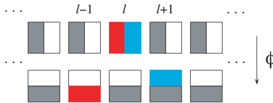
FIG. 2: Schematic representation of the action of the multibaker map (2) on several cells of its phase space.
