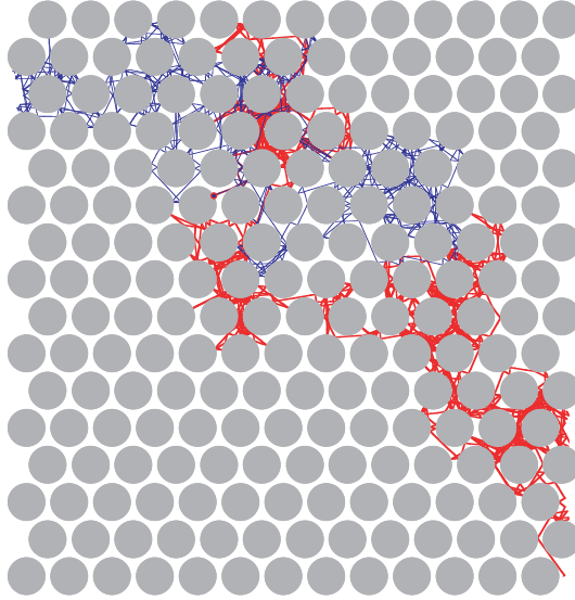
FIG. 1: Hard-disk Lorentz gas with two trajectories starting from the same position but velocities which differ by one part in a million.
