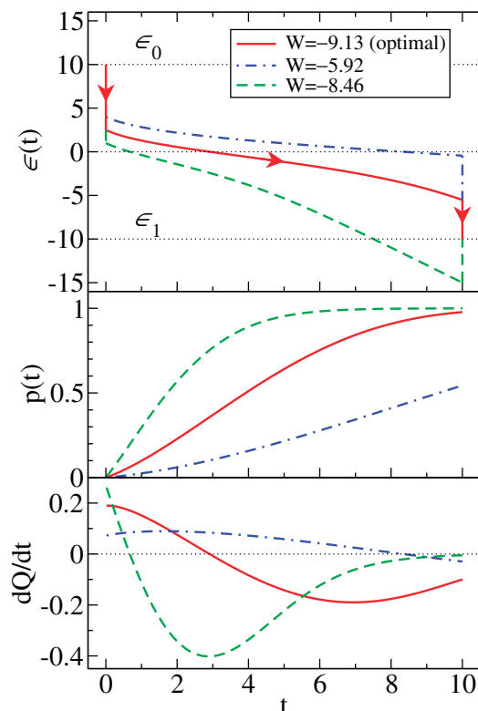
Fig. 3: (Color online) Protocol (top), occupation probability (middle), and heat flux (bottom). The energy level is lowered from \epsilon_0 = 10T to \epsilon_1 = -10T during time \tau = 10 . The red solid lines indicate optimal protocol with minimum work W = -9.13T . A protocol with a large initial jump (green dashed lines) and another protocol with a small initial jump (blue dot-dashed lines) result in higher work W = -8.58T and W = -5.92T , respectively.
