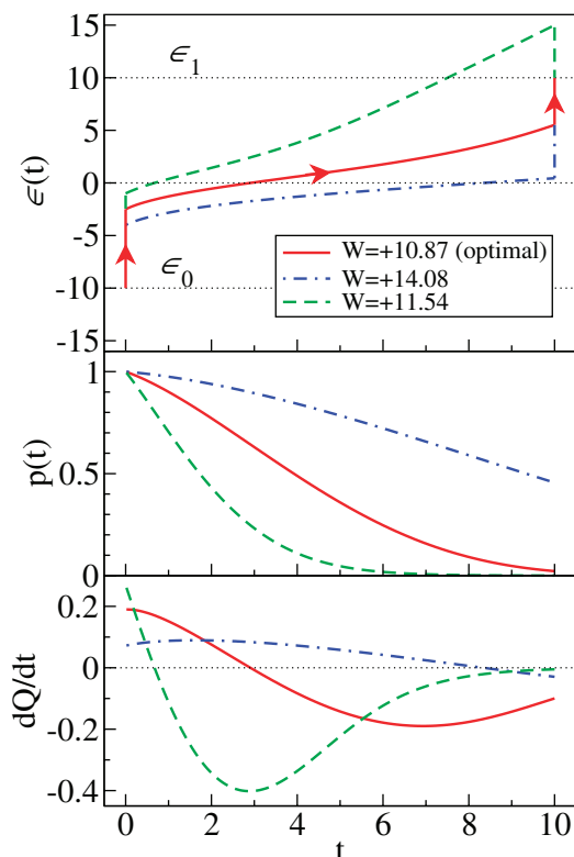
Fig. 2: (Color online) Protocol (top), occupation probability (middle), and heat flux (bottom). The energy level is raised from \epsilon_0 = -10T to \epsilon_1 = 10T during time \tau = 10 . The red solid lines indicate optimal protocol with minimum work W = 10.87T . A protocol with a large initial jump (green dashed lines) and another protocol with a small initial jump (blue dot-dashed lines) result in higher work W = 16.79T and W = 11.16T , respectively.
