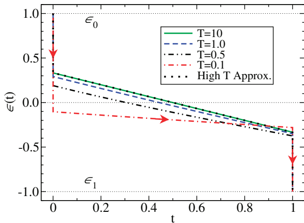
Fig. 5: (Color online) The optimal protocols for four different temperatures, T=10 (green solid line), T=1 (blue dashed line), T=0.5 (black dash-double-dotted line), and T=0.1 (red dash-dotted line). The energy level is lowered from \epsilon_0 = 1 to \epsilon_1 = -1 .
