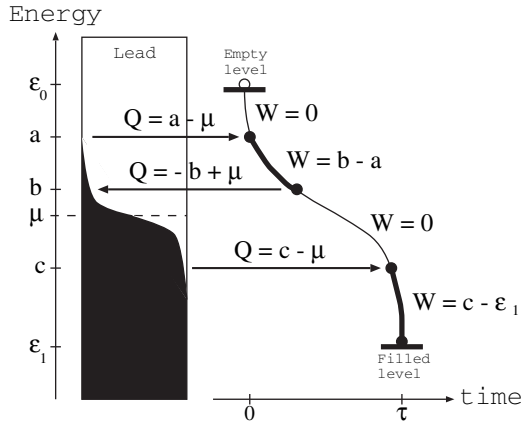
Fig. 1: The model: a single-level quantum dot interacts with a metallic lead. The level is initially at \varepsilon_0 in thermal equilibrium but is lowered to \varepsilon_1 in a finite time \tau according to a given protocol \varepsilon(t) . We depict a typical trajectory for such a process along which heat is exchanged and work is extracted. Work and heat are obtained by averaging over all possible trajectories associated with this process.
