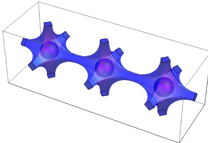
Figure 4. Finite horizon can be achieved in a three-dimensional lattice, provided that the spheres are allowed to overlap. Here the available space for diffusing particles is shown for the parameter values \rho_{\text{out}} = 0.65 and \rho_{\text{in}} = 0.15 (in the FH1 region) in an unfolded channel.
